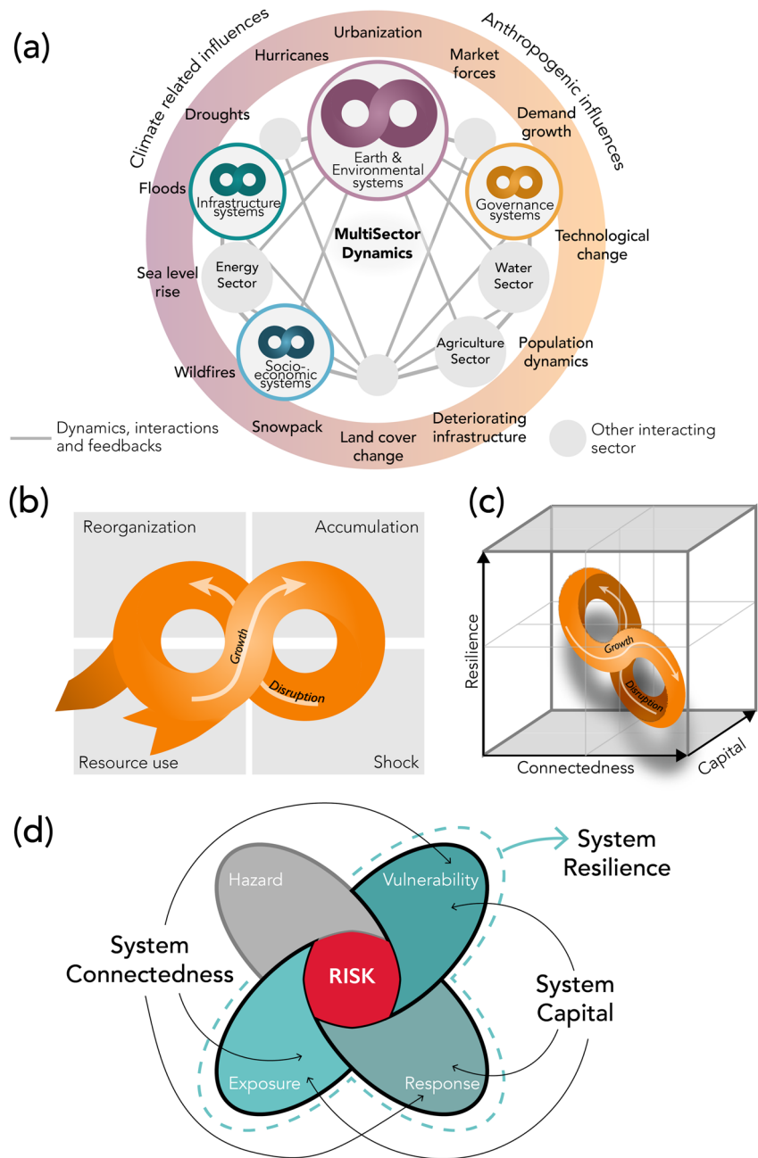
Figure 3. Key concepts for MultiSector Dynamics. (a) MultiSector Dynamics are shaped by co-evolving human and natural influences that emerge across interactions across sectors and systems. The energy, water, and agricultural sectors are shown as examples and other non-labeled sectors are shown in gray circles. (b) Adaptive cycles of growth and disruption of a complex system adapted from (Holling, 1985; Holling & Gunderson, 2002). (c) Illustration of the relationships between the adaptive cycle for a system and its key properties (resilience, connectedness, and capital). (d) Conceptual linkage between the risk and resilience for complex human-Earth systems.
